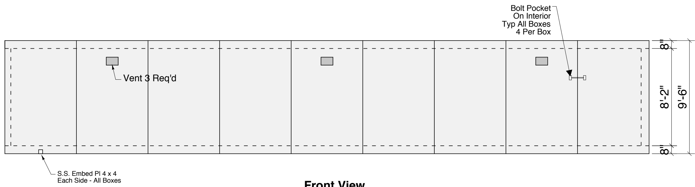
Front View
