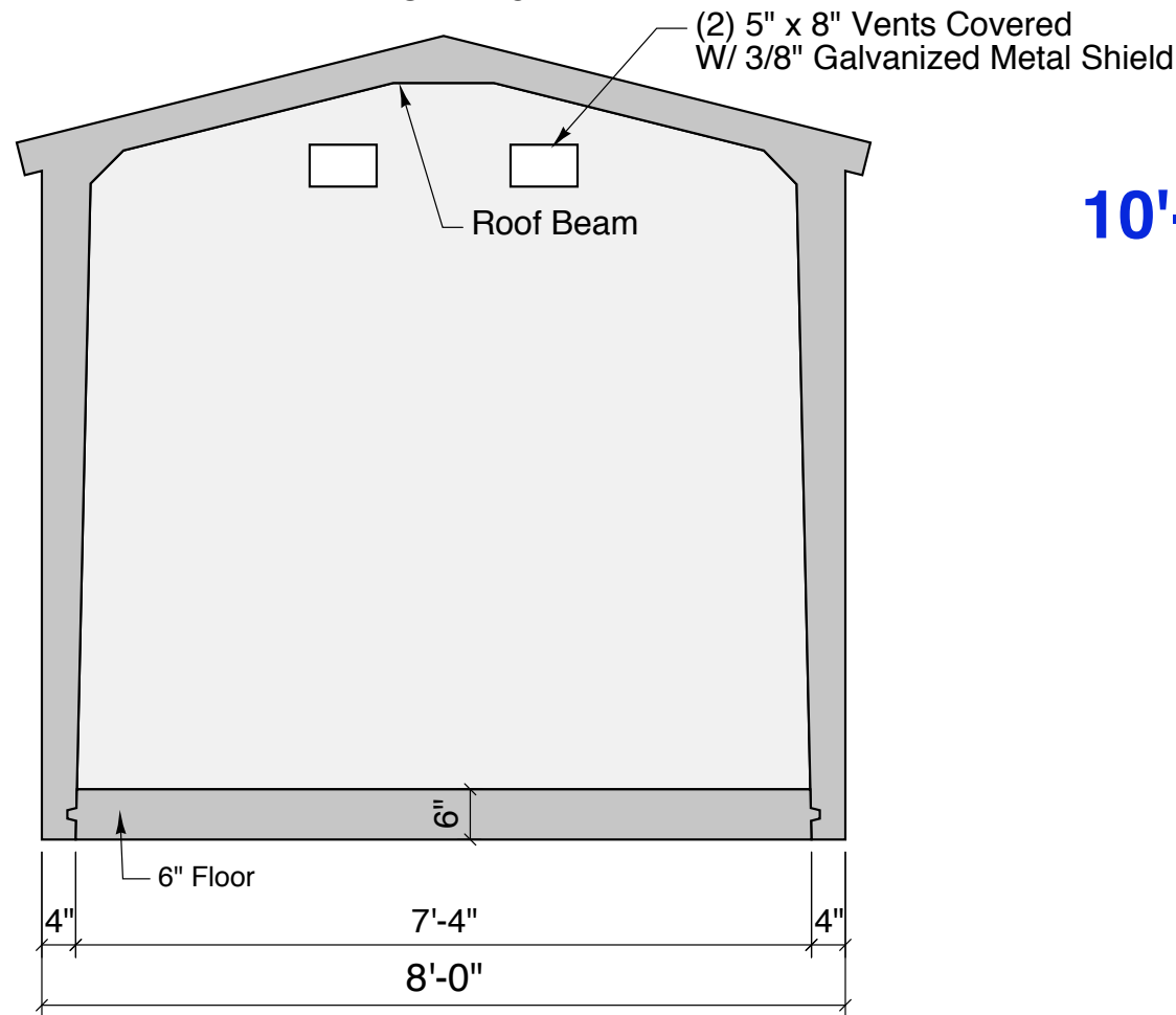
Section Thru Hut
