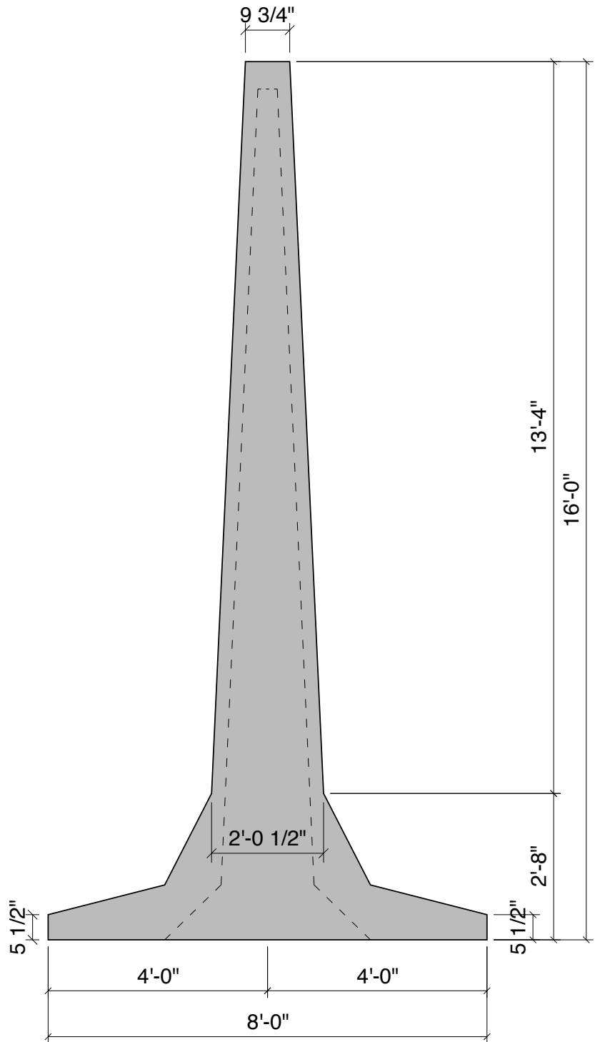
End View
